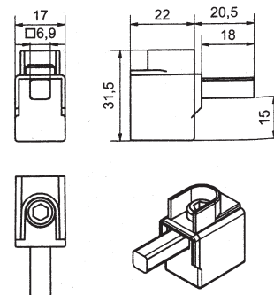
KKL 1x120T3
